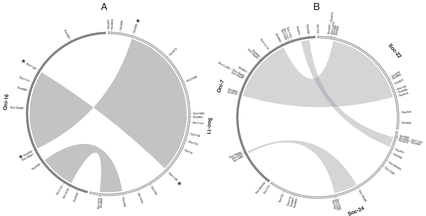
Fig. 3. Circular ideograms, generated using CIRCOS v 0.66, showing putative intra- and inter-chromosomal rearrangements that occurred since red drum and Nile tilapia diverged from a common ancestor. A, an inferred chromosomal rearrangement involving syntenic groups on red drum linkage group 11 ( Soc-11 ) and Nile tilapia chromosome 16 ( Oni-16 ). Ribbons linking chromosomes represent regions of shared synteny. The two syntenic regions derived from Soc-11 are inverted on Oni-16 relative to their position on Soc-11 . Asterisks indicate the ends of relocated syntenic blocks. B, an inferred fusion involving syntenic groups on two red drum chromosomes ( Soc-22 and Soc-24 ) occurring on a single Nile tilapia chromosome ( Oni-7 ). A fusion in the Nile tilapia lineage is inferred because Soc-22 and Soc-24 are syntenic to separate chromosomes in the other three comparison species (data not shown). The two syntenic regions from Soc-24 flank a single syntenic region from Soc-22 on Oni-7 , suggesting that a fusion was followed by one or more intra-chromosomal rearrangements.
